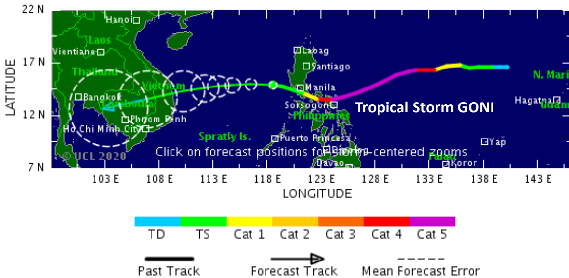
Figure 3: The moving of Tropical Storm Goni towards the Mekong region, observed on 02 November 2020.
