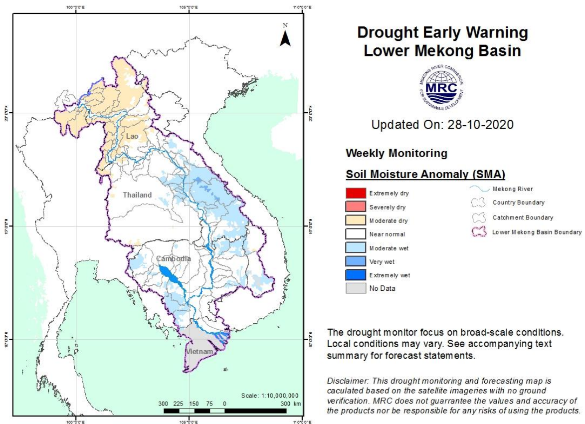
Figure 13: Weekly Soil Moisture Anomaly from Oct 22-28.
