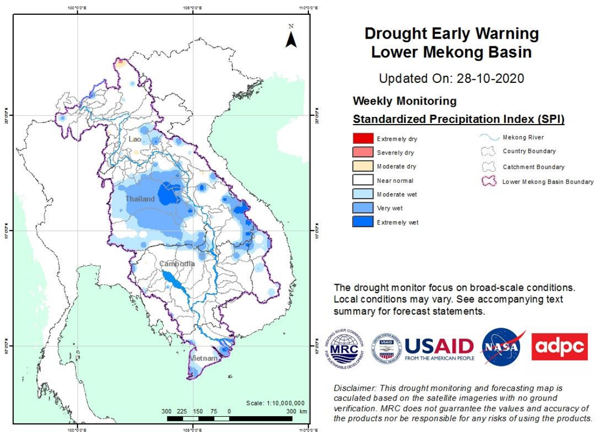
Figure 12: Weekly standardised precipitation index from Oct 22-28.
