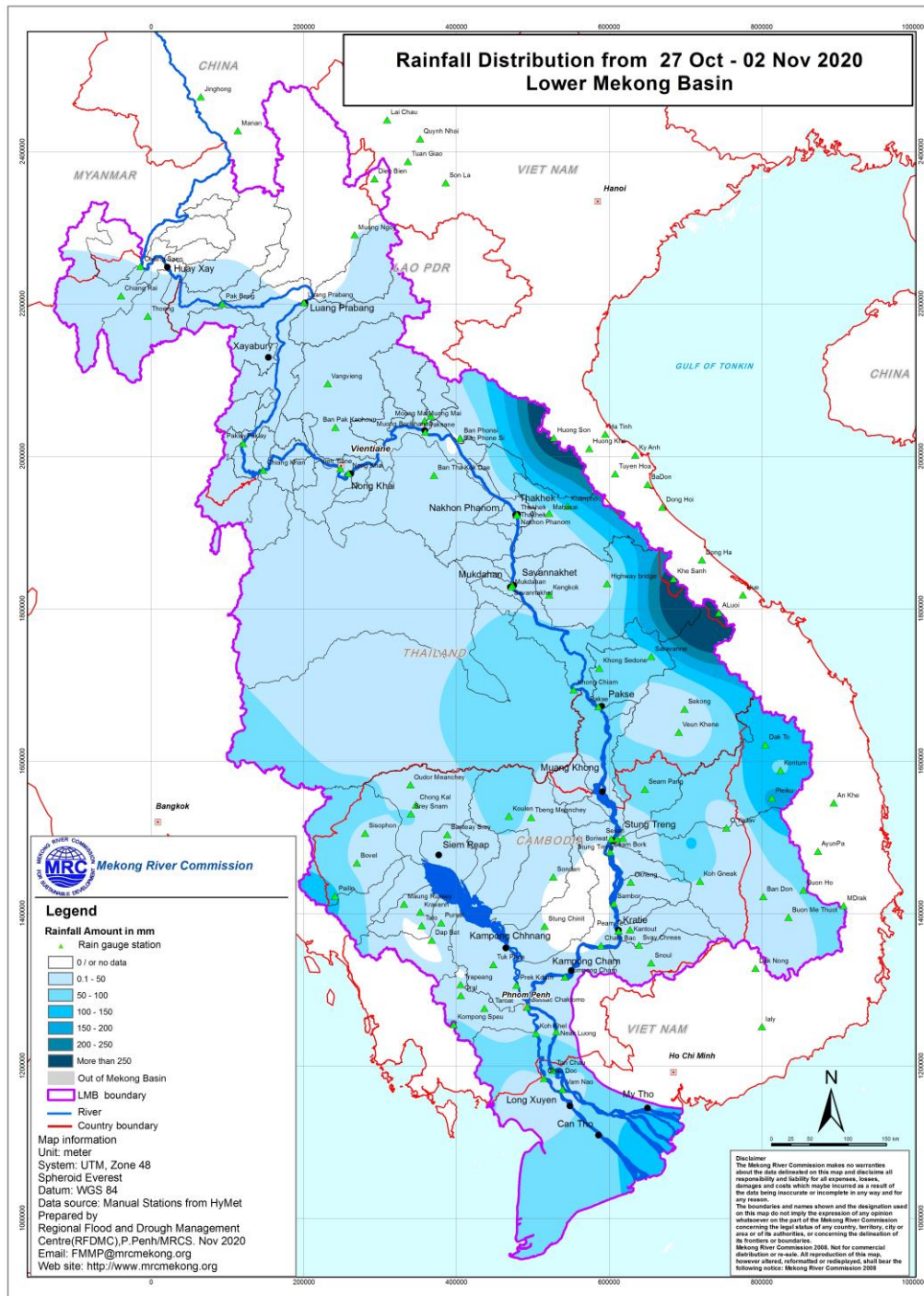
Figure 5: Weekly rainfall distribution over the LMB.
