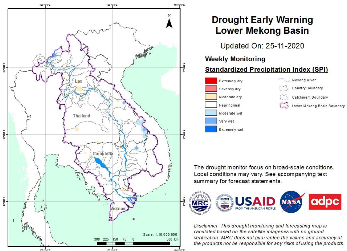
Figure 11: Weekly standardised precipitation index from Nov 19–25.
