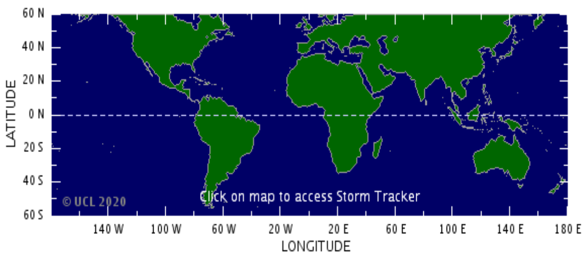
Figure 3: No tropical storm risk observed on 30 November.
