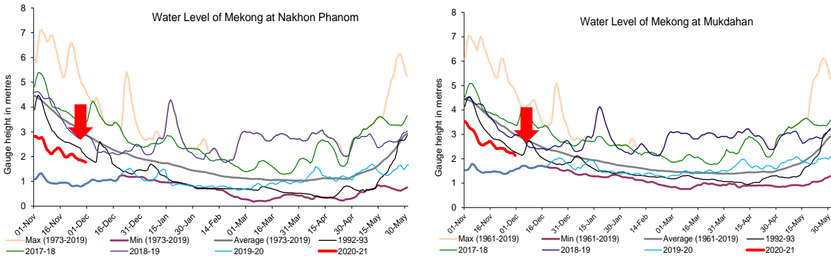
Figure 7: Water levels at Nakhon Phanom and Mukdahan of Thailand.
