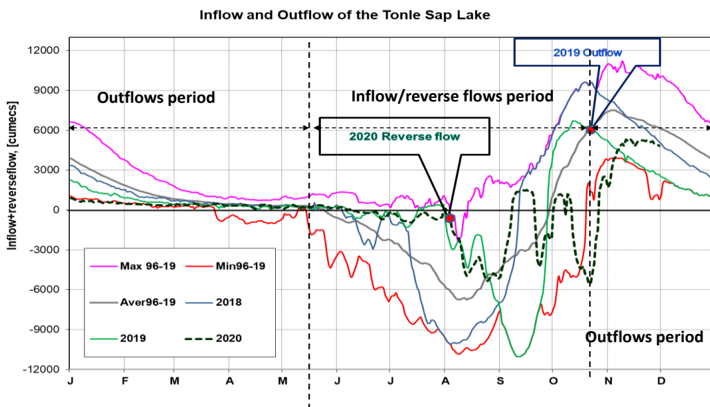
Figure 9: Seasonal change of inflows and outflows of Tonle Sap Lake.
