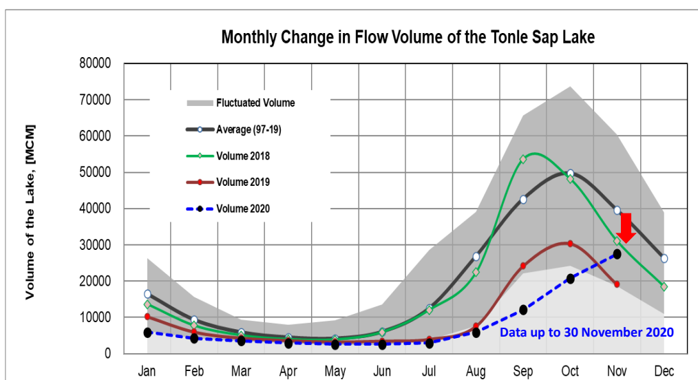
Figure 10: The seasonal change in monthly flow volume of Tonle Sap Lake.
