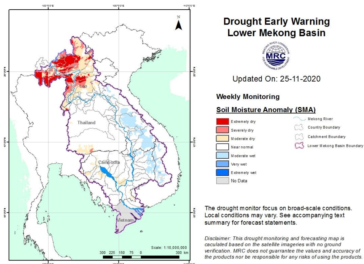
Figure 12: Weekly Soil Moisture Anomaly from Nov 19 to 25.
