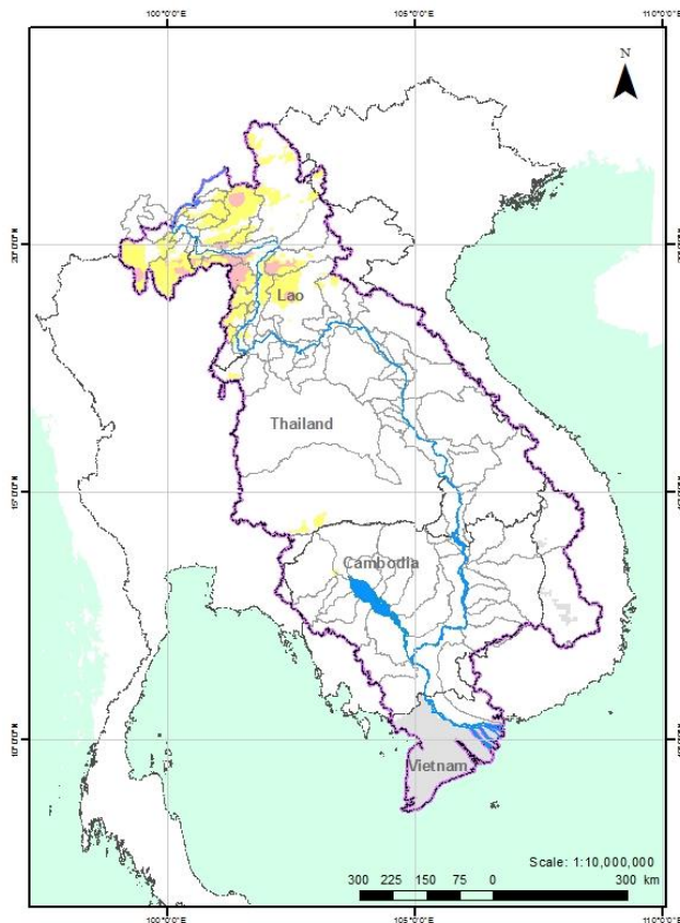
Figure 13: Weekly Combined Drought Index during Nov 19-25.
