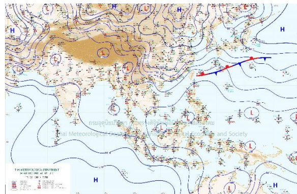
Figure 2: Weather map for 15 th Oct 2018
