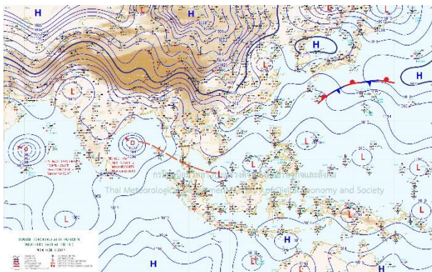
Figure 1: Weather map for 09 th Oct 2018
