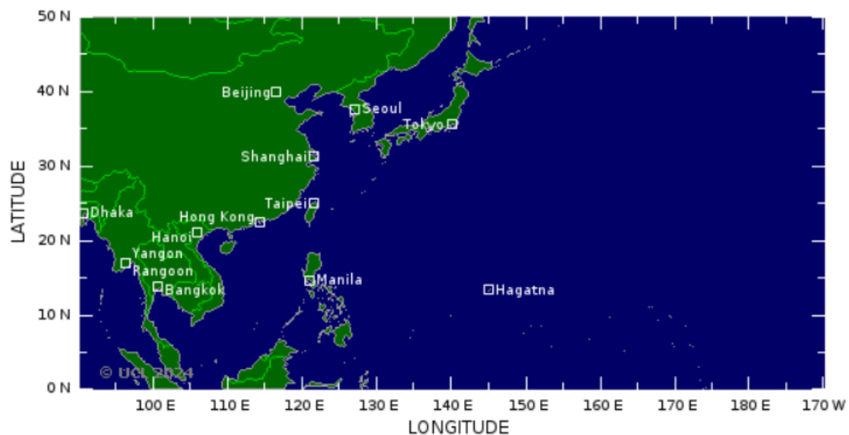
Figure 3: No tropical storm risk observed on 11 March 2024
