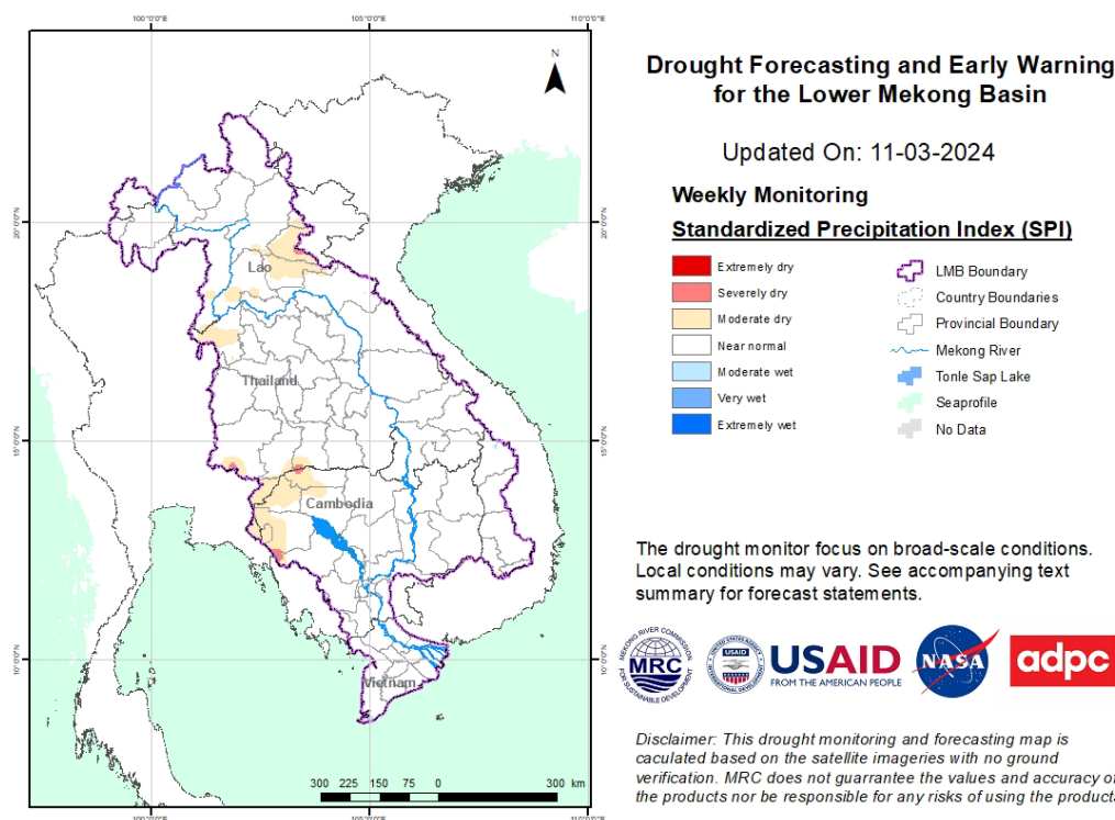
Figure 9: Weekly standardised precipitation index from March 5 to 11.
