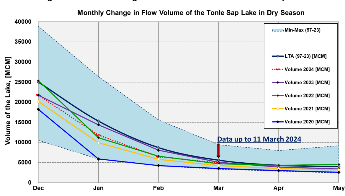
Figure 8. The seasonal change in monthly flow volume of Tonle Sap Lake.
