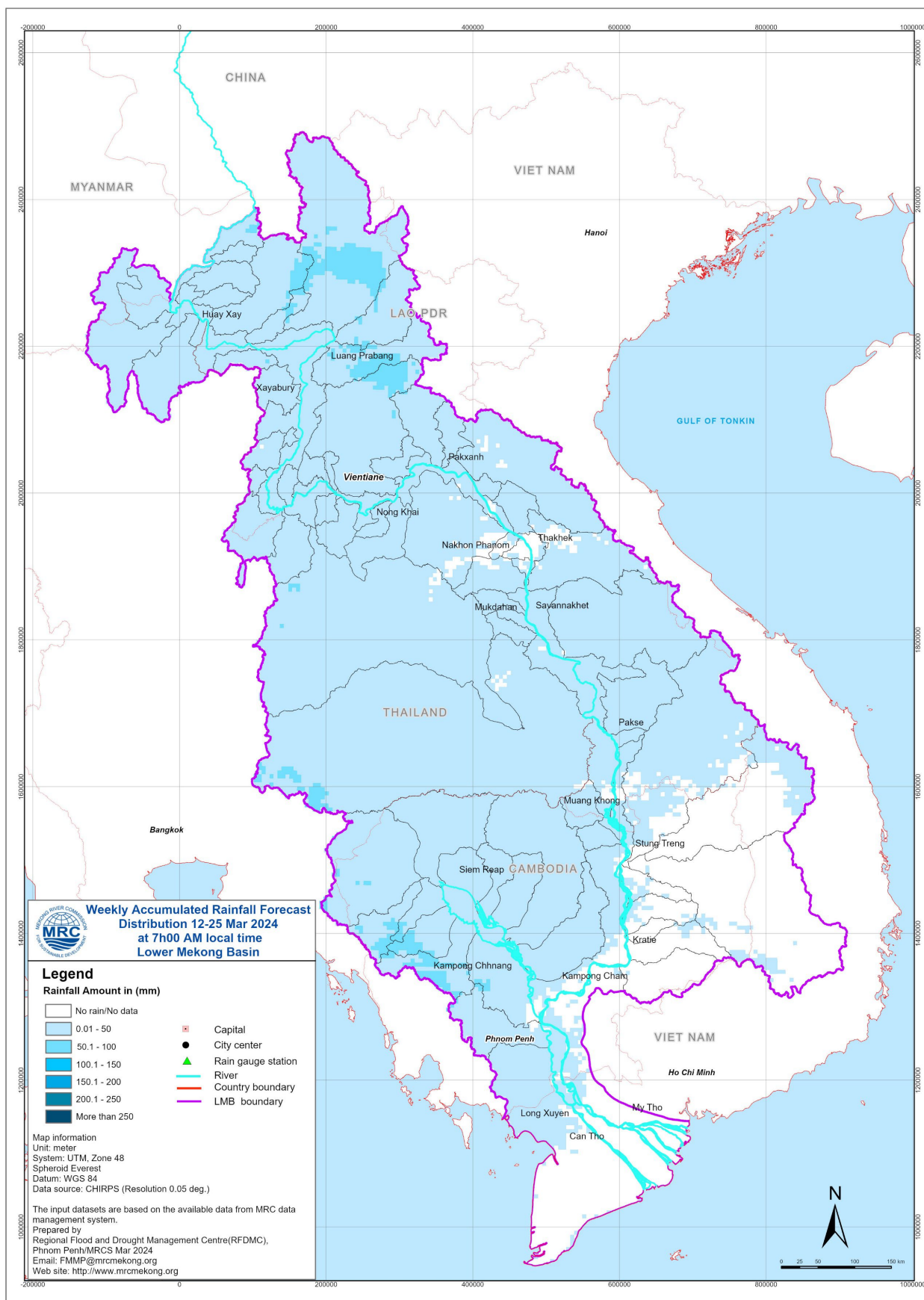
Figure 12: Accumulated rainfall forecast from CHIRP-GFS (12 - 25 March 2024)
