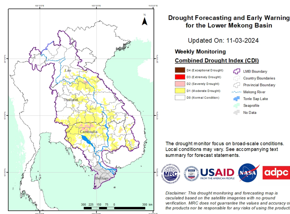
Figure 11: Weekly Combined Drought Index from March 5 to 11.
