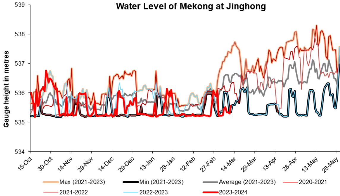
Figure 6. Water level at the Jinghong hydrological station up to 11 March 2024.
