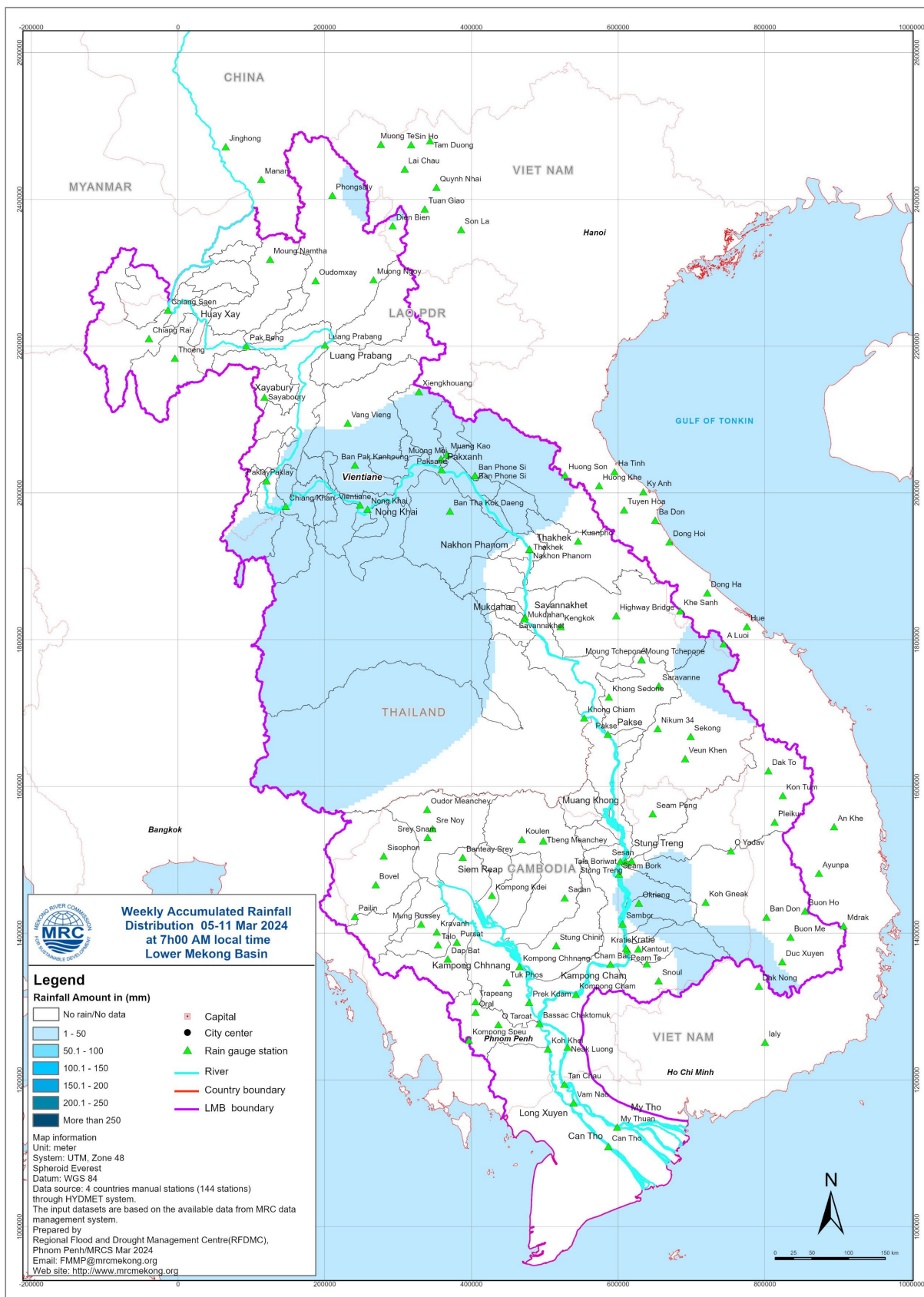
Figure 4: Weekly rainfall distribution over the LMB during 05 – 11 March 2024
