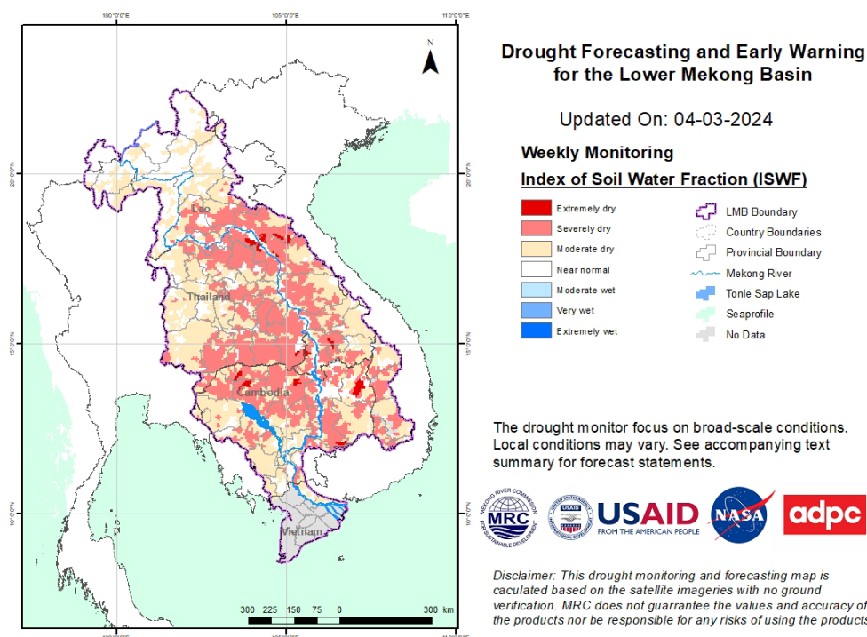
Figure 10: Weekly Index of Soil Water Fraction from March 5 to 11.
