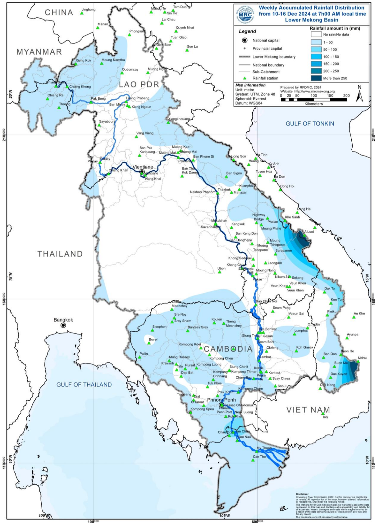
Figure 4: Weekly rainfall distribution over the LMB during 10 – 16 Dec 2024
