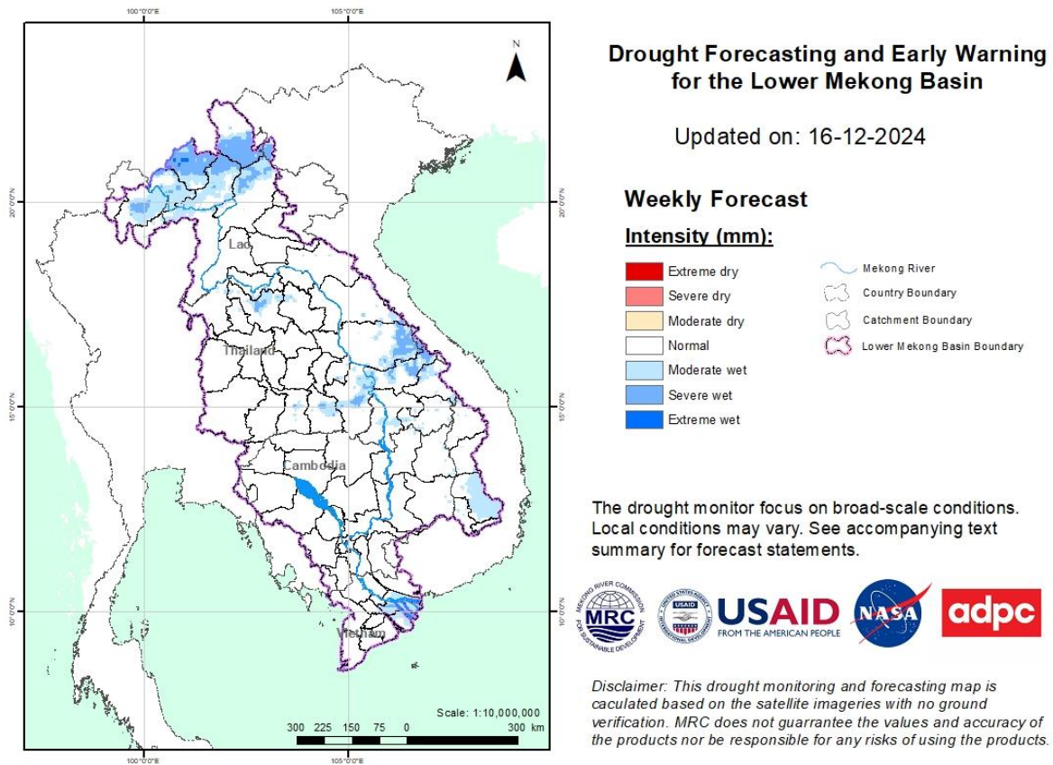
Figure 9: Weekly standardized precipitation index from 10 - 16 December.
