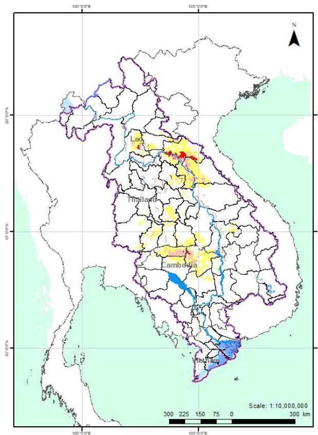
Figure 11: Weekly Combined Drought Index from 10 - 16 December.
