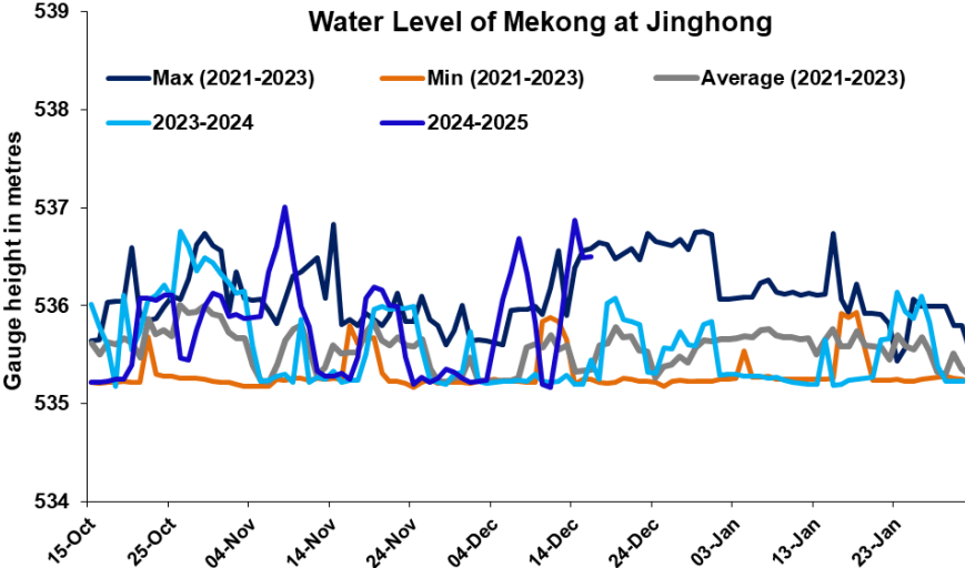
Figure 6. Water level at the Jinghong hydrological station up to 16 December 2024.
