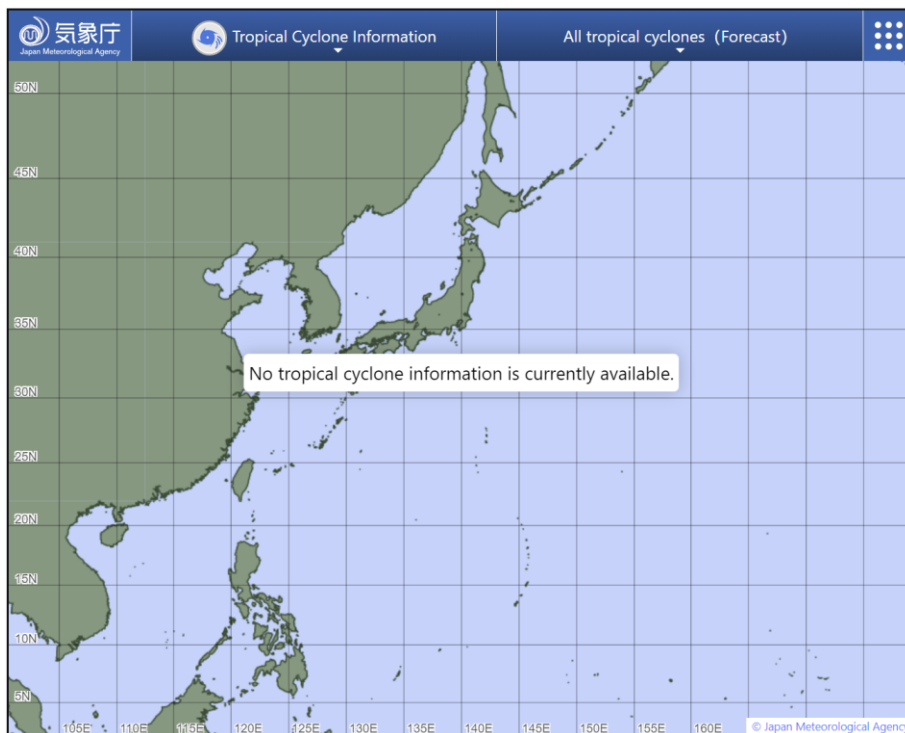
Figure 3: One tropical storm risk observed on 16 December 2024
