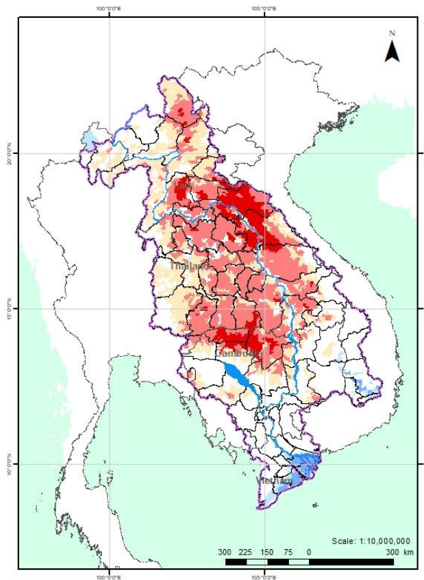
Figure 10: Weekly Index of Soil Water Fraction from 10 - 16 December.
