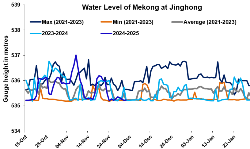
Figure 6. Water level at the Jinghong hydrological station up to 02 December 2024.
