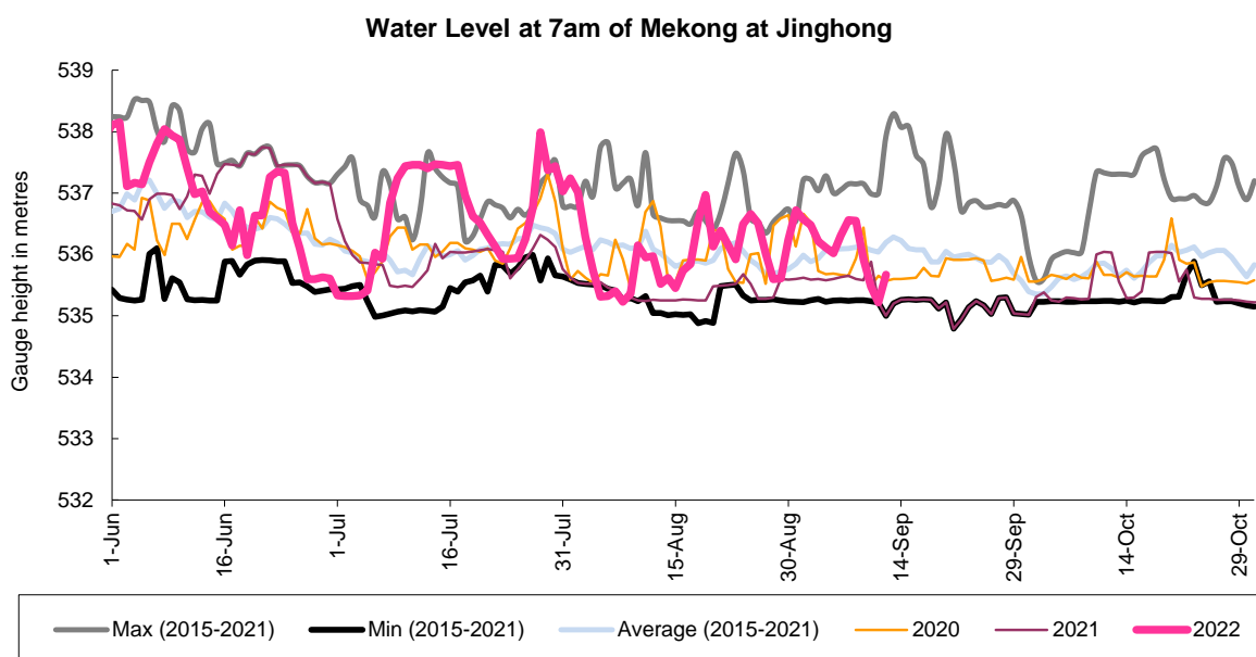
Figure 7. Water level at the Jinghong hydrological station up to 12 September 2022.
