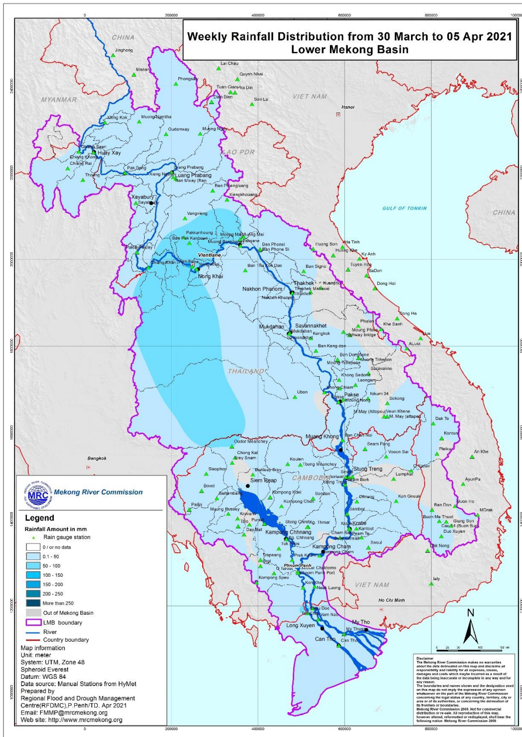
Figure 5: Weekly rainfall distribution over the LMB during 30 Mar – 5 Apr 2021.
