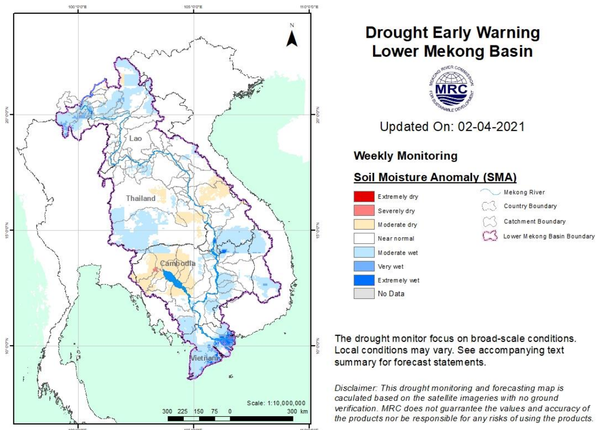
Figure 13: Weekly Soil Moisture Anomaly from 27 Mar to 02 Apr 2021.
