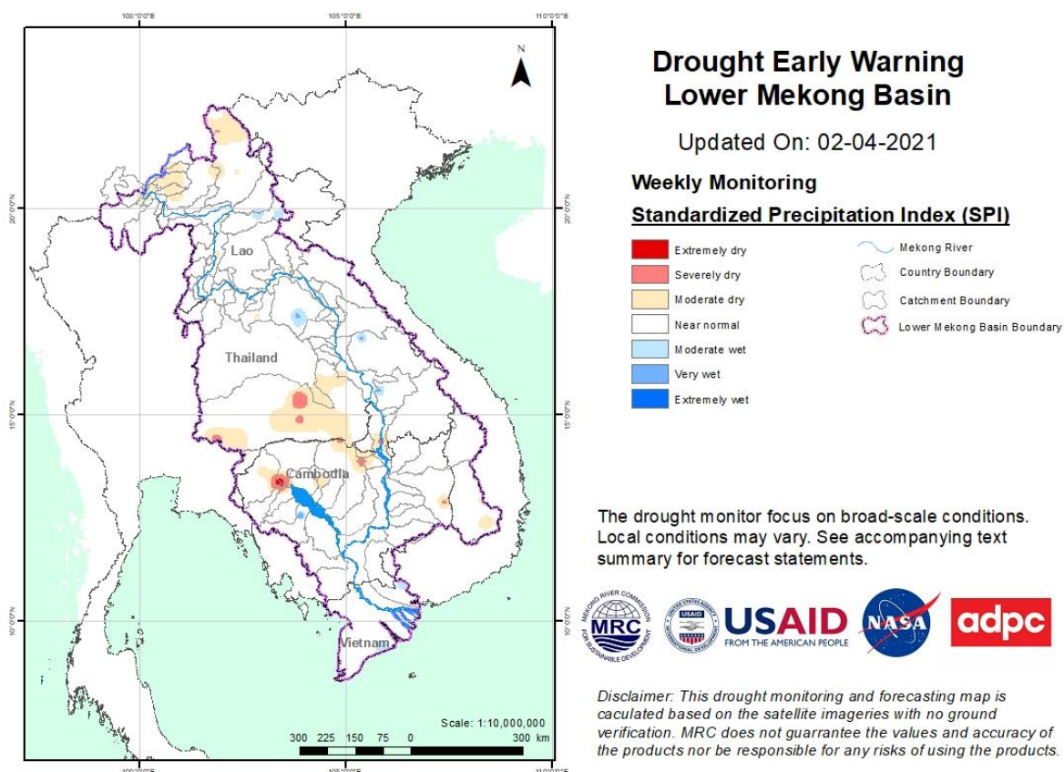
Figure 12: Weekly standardized precipitation index from 27 Mar to 02 Apr 2021.
