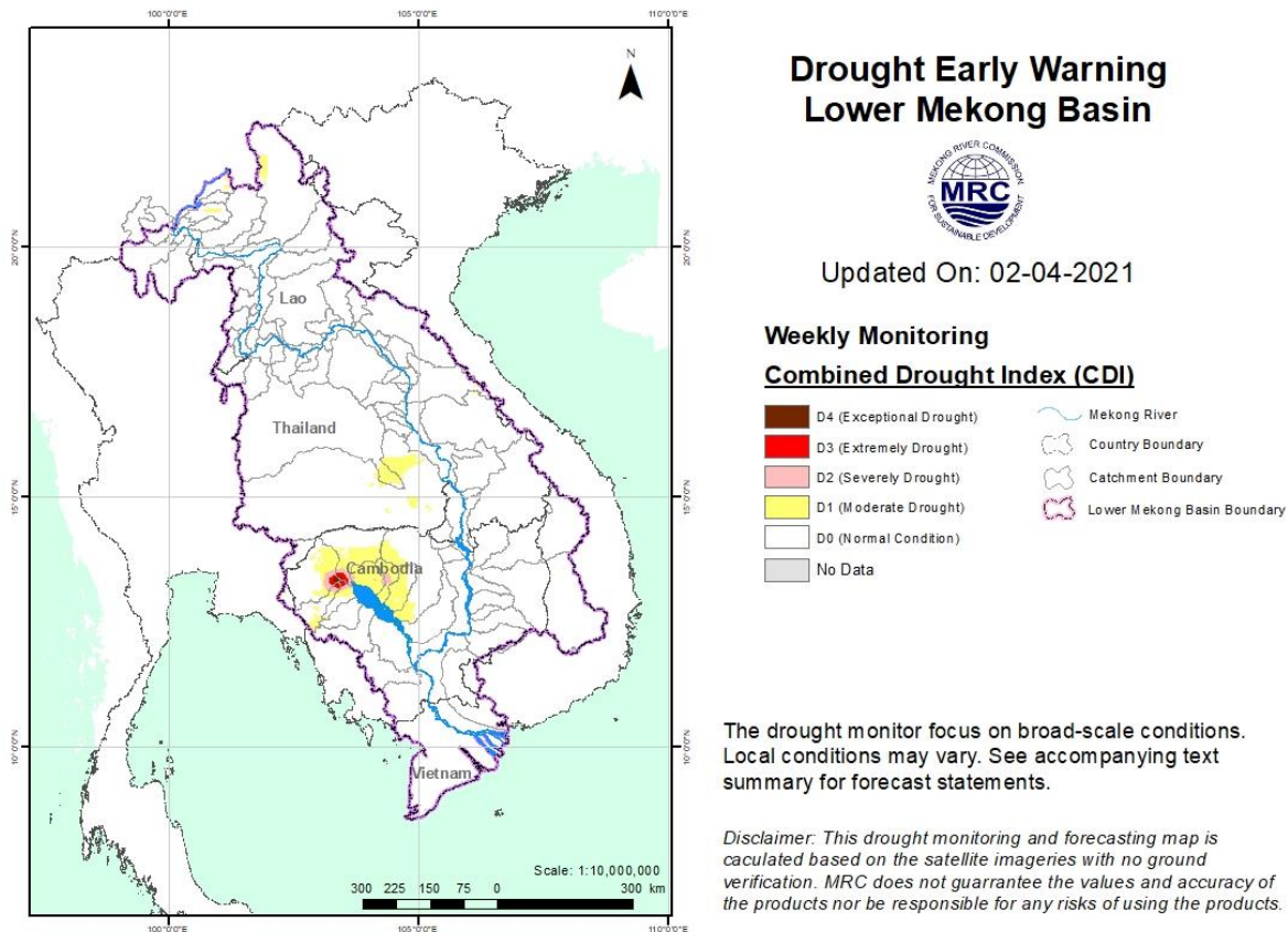
Figure 14: Weekly Combined Drought Index from 27 Mar to 02 Apr 2021.
