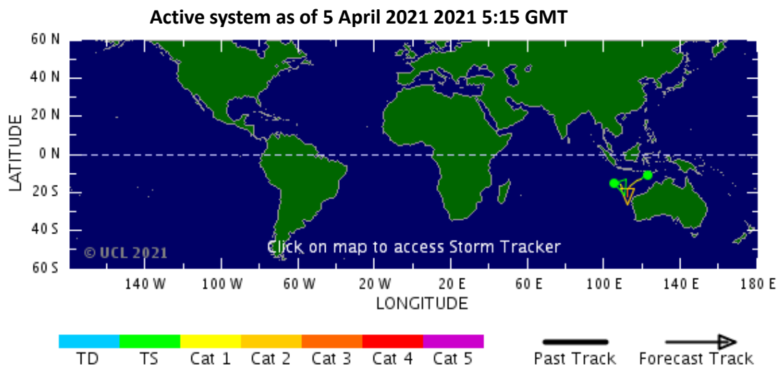
Figure 3: A Tropical Depression risk observed on 5 April 2021.
