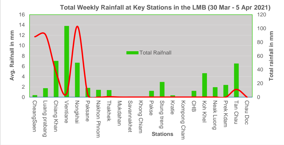
Figure 4: Weekly total rainfall at key stations in the LMB during 30 March-5 April 2021.
