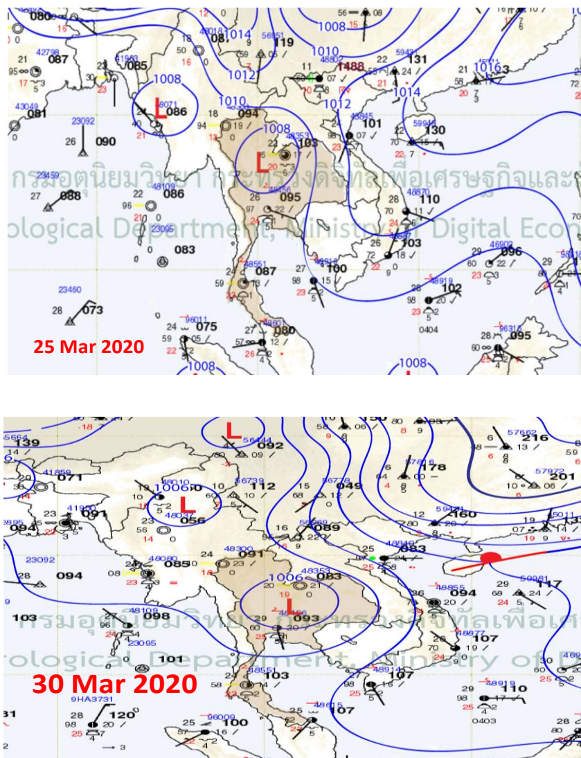
Figure 1: Summary of weather condition over the LMB from 25 and 30 March 2020
