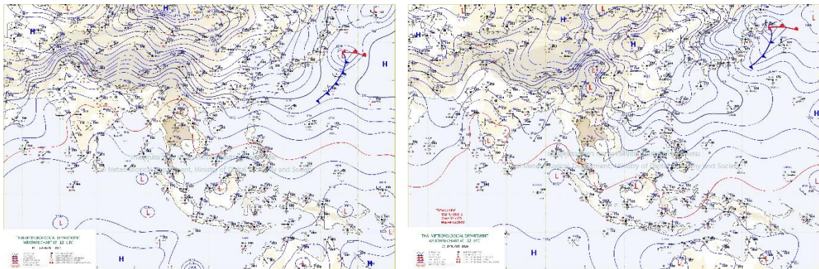
Figure 1: Summary of weather condition over the LMB from 15 and 20 Jan 2020
