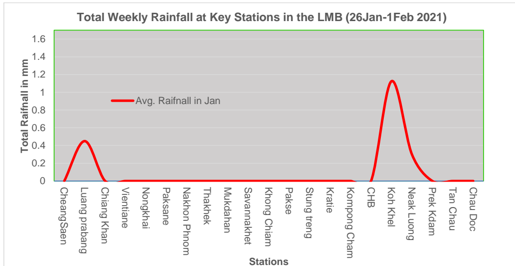
Figure 4: Weekly total rainfall at key stations in the LMB during 26 Jan-1 Feb 2021.
