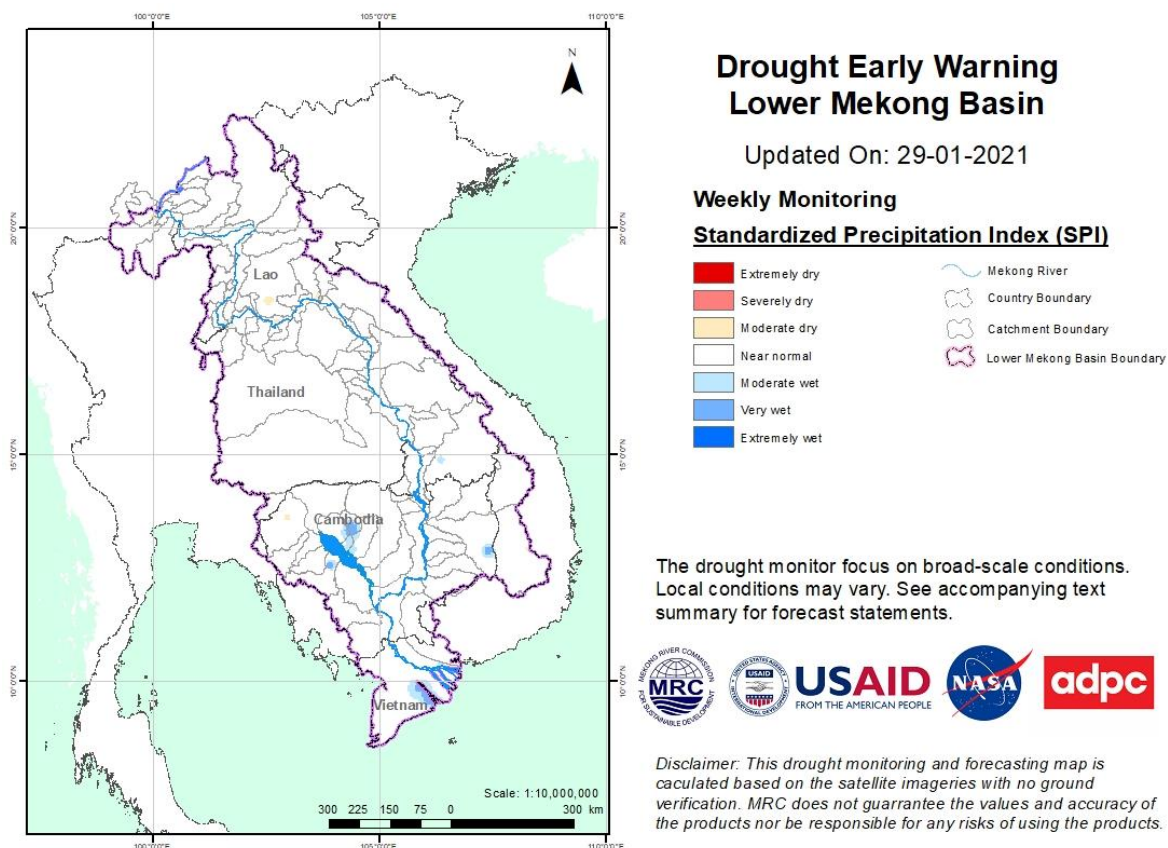
Figure 12: Weekly standardized precipitation index from 23 to 29 Jan 2021.
