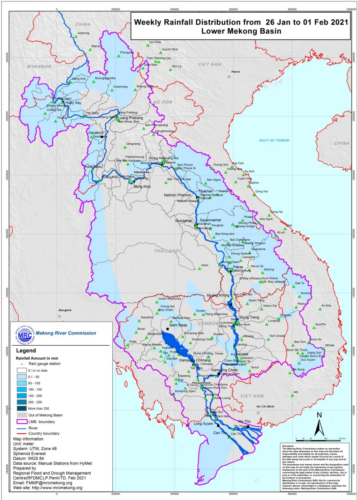
Figure 5: Weekly rainfall distribution over the LMB during 26 Jan-1 Feb 2021.
