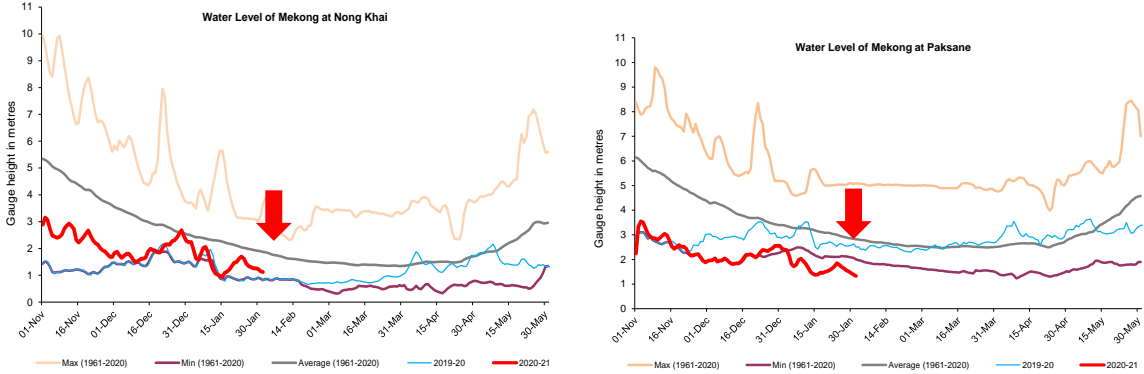
Figure 7: Water levels at Paksane of Lao PDR.
