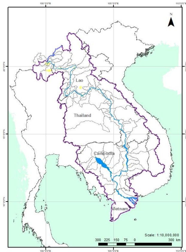
Figure 14: Weekly Combined Drought Index from 23 to 29 Jan 2021.
