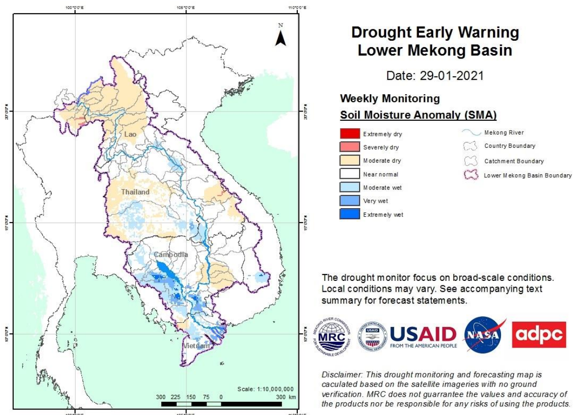
Figure 13: Weekly Soil Moisture Anomaly from 23 to 29 Jan 2021.
