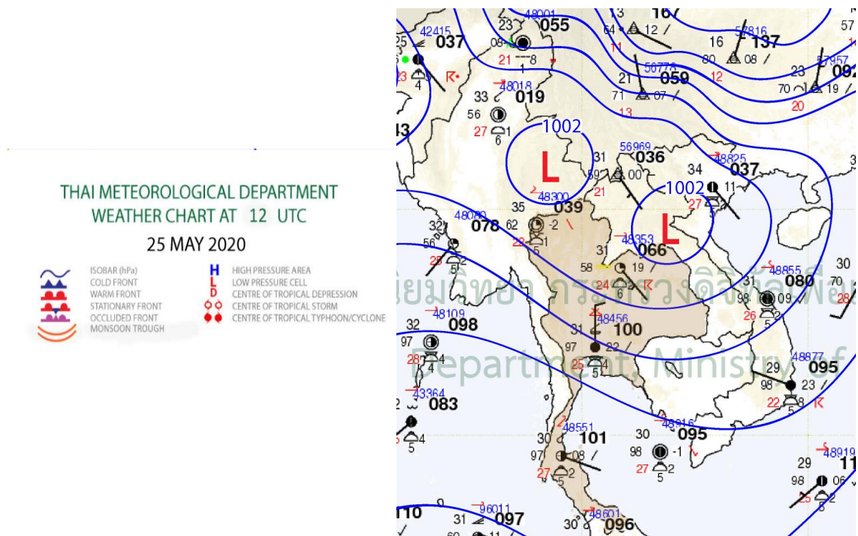
Figure 1 Summary of weather condition over the LMB on 25 May 2020
