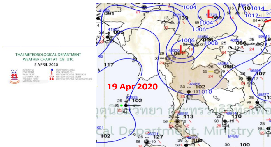
Figure 1: Summary of weather condition over the LMB from 15 and 19 April 2020
