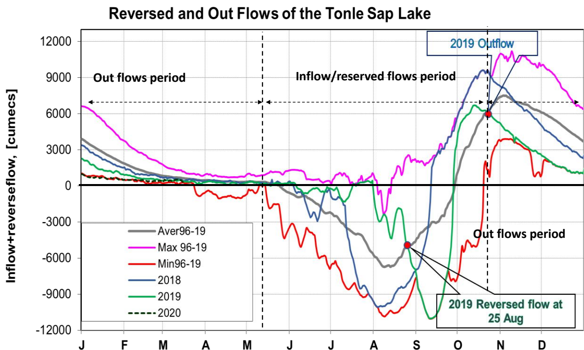
Figure 3 The seasonal change of inflow/reversed flows of the Tole Sap Lake
