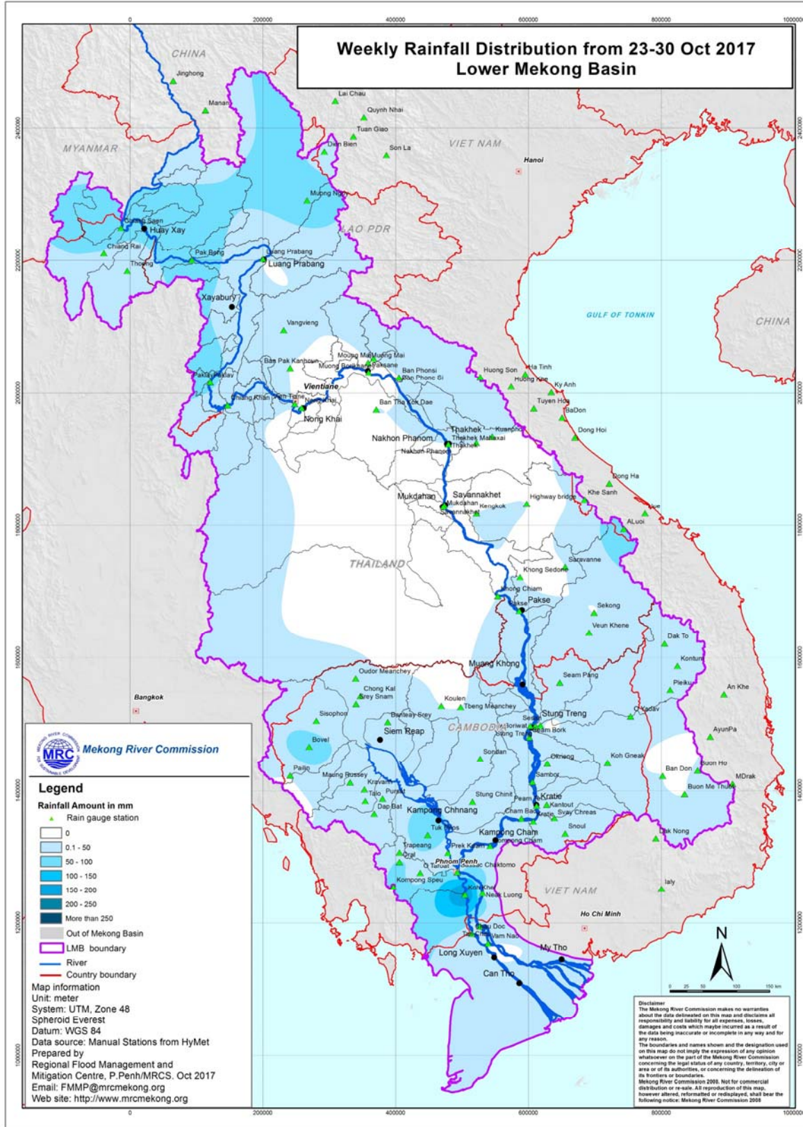
Figure 2: Weekly Rainfall Distribution over the LMB from 23 rd – 30 th October 2017
