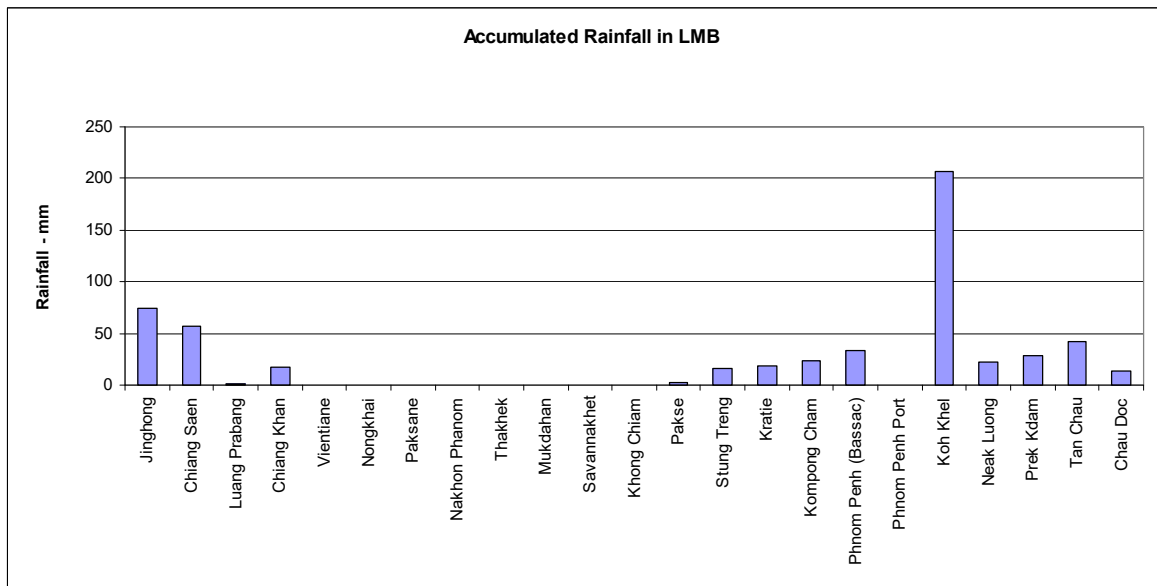
Figure 1: Accumulated Rainfall Distribution over the LMB from 23 rd – 30 th October 2017
