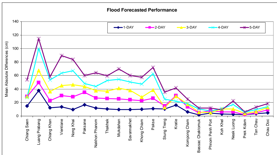
Figure B1: Average flood forecast accuracy along the Mekong mainstream (from 21 st – 28 th August 2017)
