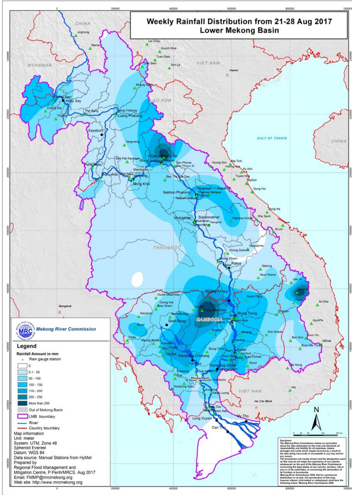
Figure 2: Weekly Rainfall Distribution over the LMB from 21 st – 28 th August 2017
