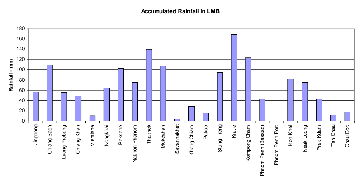
Figure 1: Accumulated Rainfall Distribution over the LMB from 21 st – 28 th August 2017
