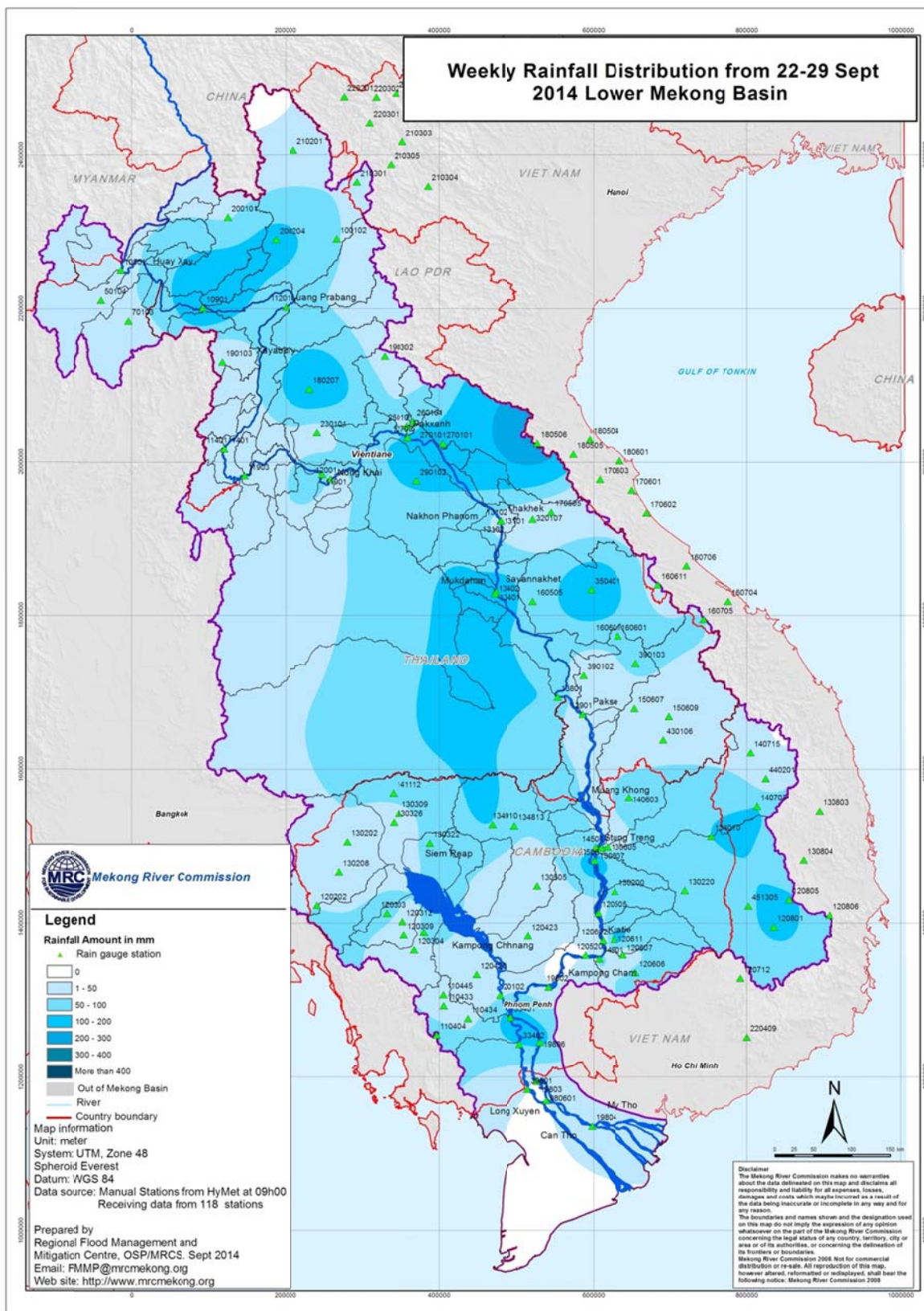
Figure 3: Weekly Rainfall Distribution from 22 nd – 29 th September 2014 over the LMB
