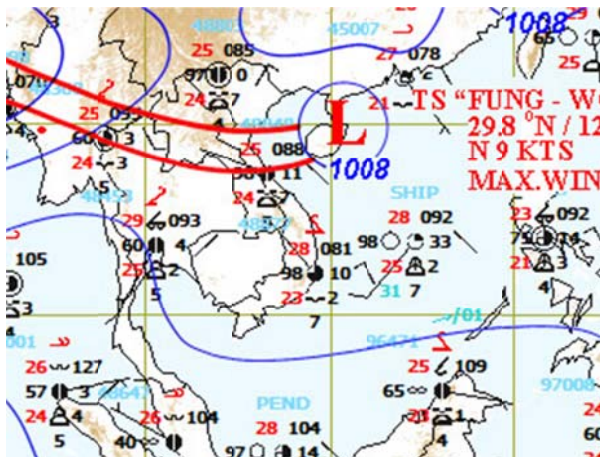
Figure 1: Weather map for 22 nd September 2014
