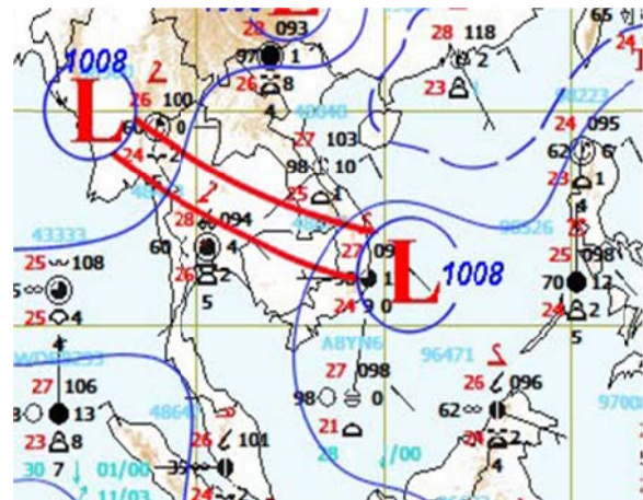
Figure 2: Weather map for 28 th September 2014
