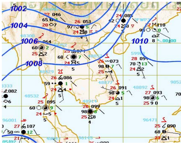
Figure 1: Weather map for 08 th July 2013
