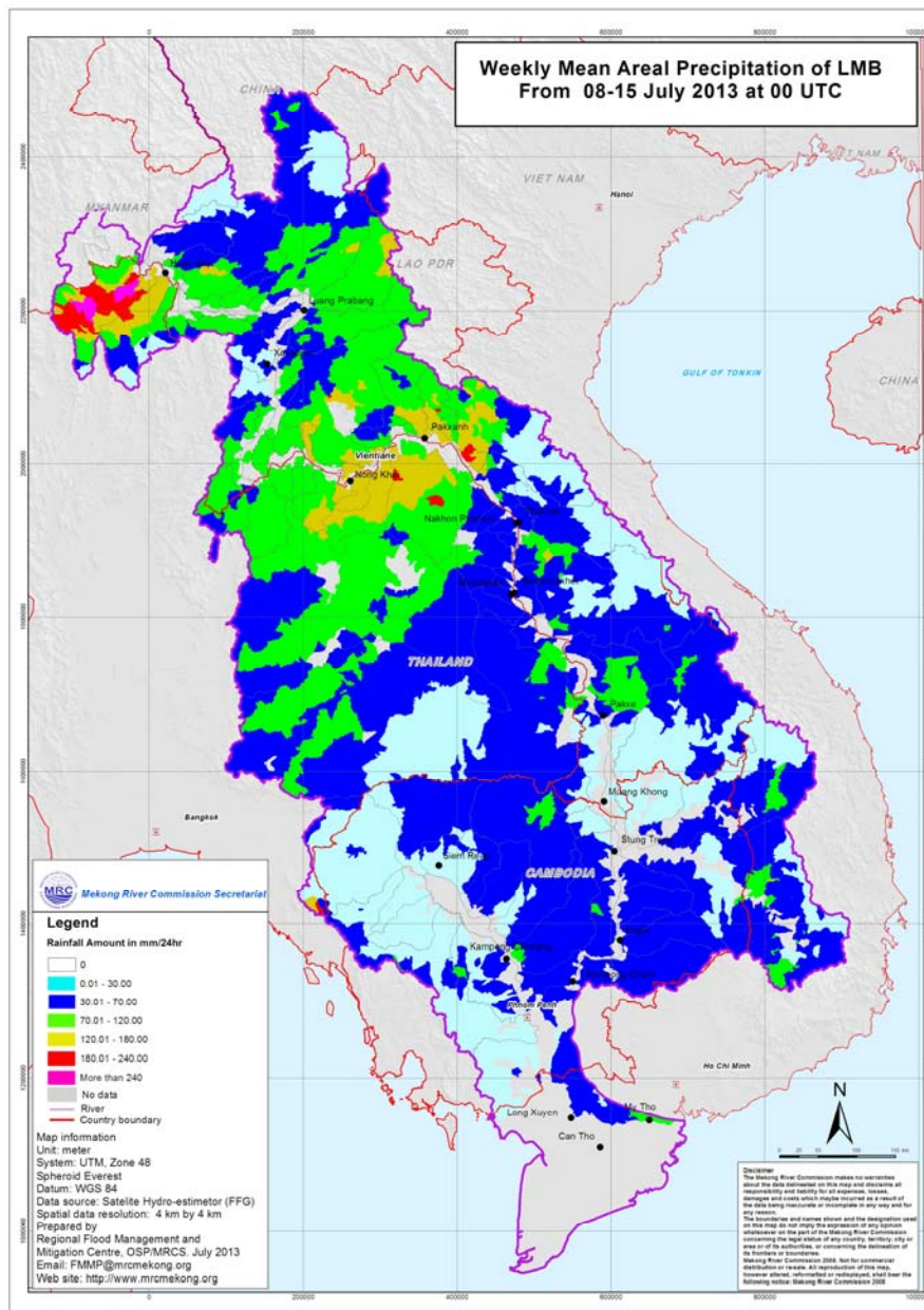
Figure 3: Rainfall distribution over the LMB, covering the week 08 th July – 15 th July, 2013
