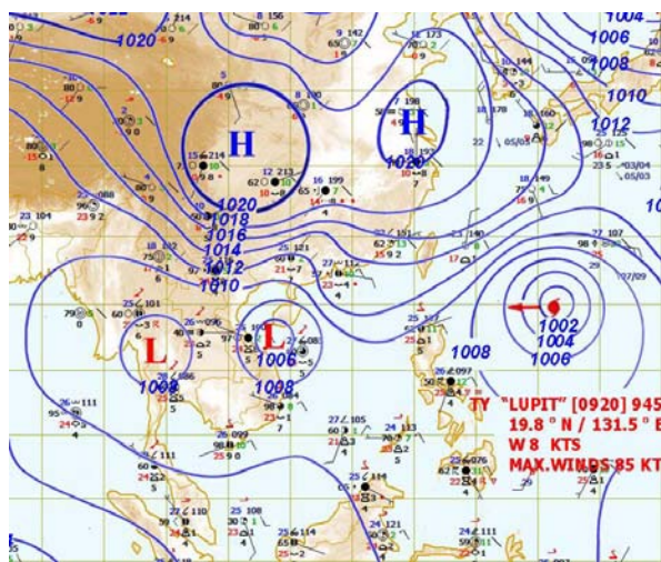
Figure 1: Weather map for 19 October 2009
