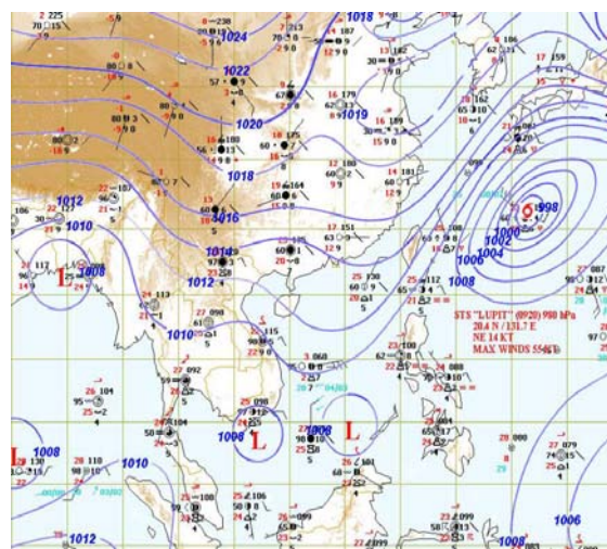
Figure 2: Weather map for 25 October 2009
